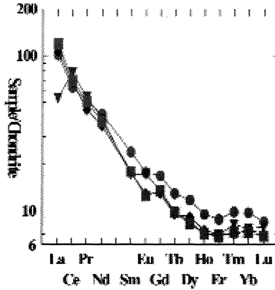
Figure 9. Chondrite-normalized rare earth element patterns for rocks. Normalizing values from Boynton (1984). Filled circle; basaltic andesite, inverted triangle; tüf, square; dasite, diamond; andesite.
